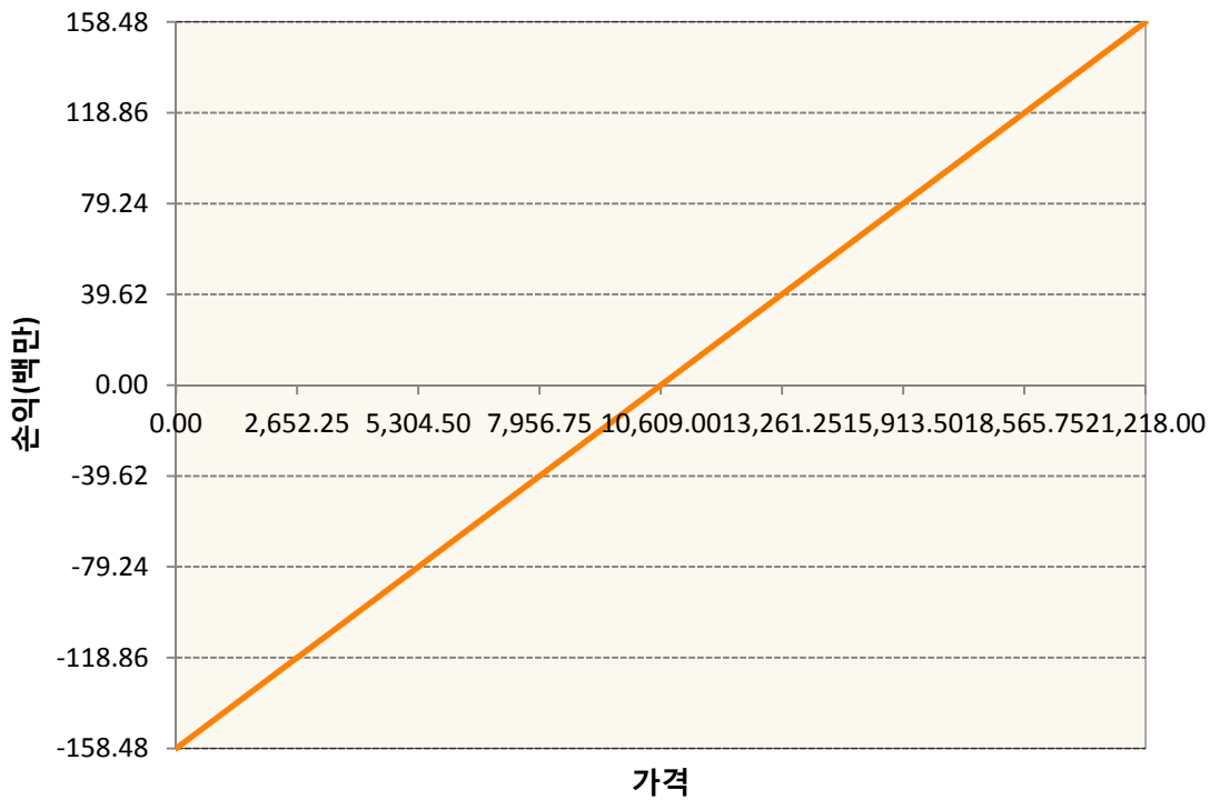
HCF0-HSCEI Futures Jan20
