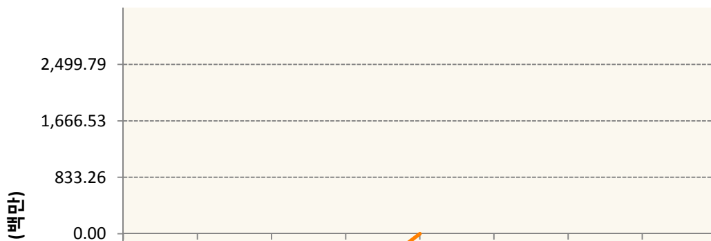
OESXZ8-P3200-EURO STOXX 50
