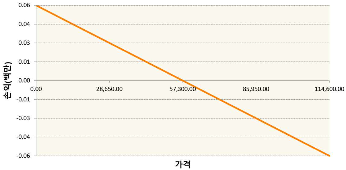
KR4146T20005-2023-02 KB금융개별선물
