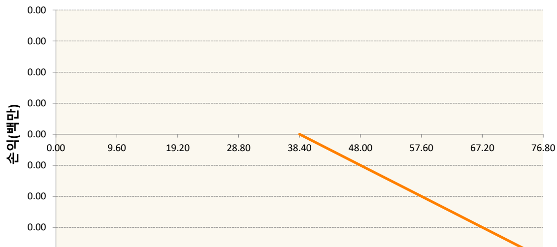
OESXU2-C3750-EURO STOXX 50
