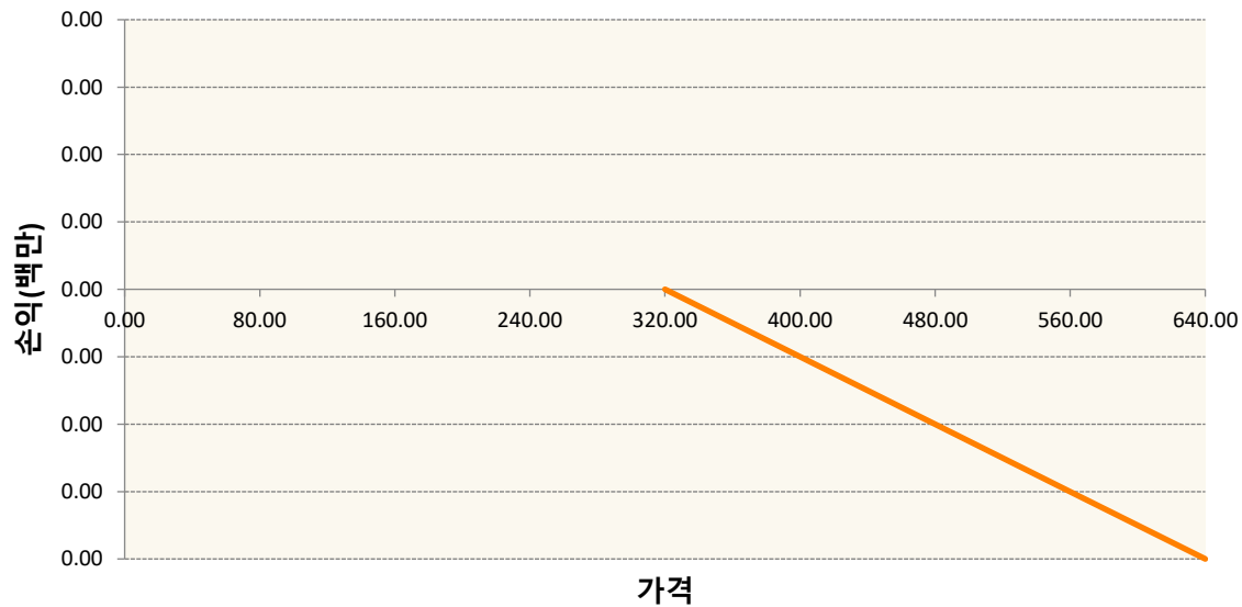
KR4201S83206-2022-08 콜320
