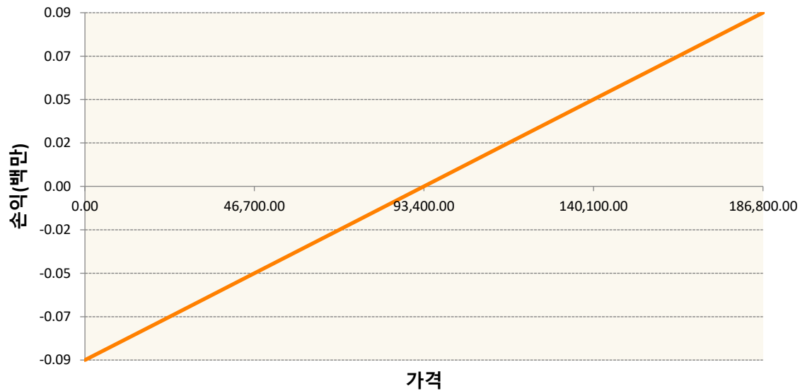
KR4150S80003-2022-08 SK하이닉스개별선물
