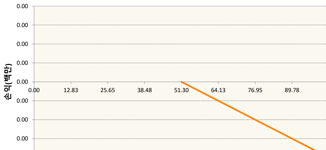
OESXN2-C3450-EURO STOXX 50
