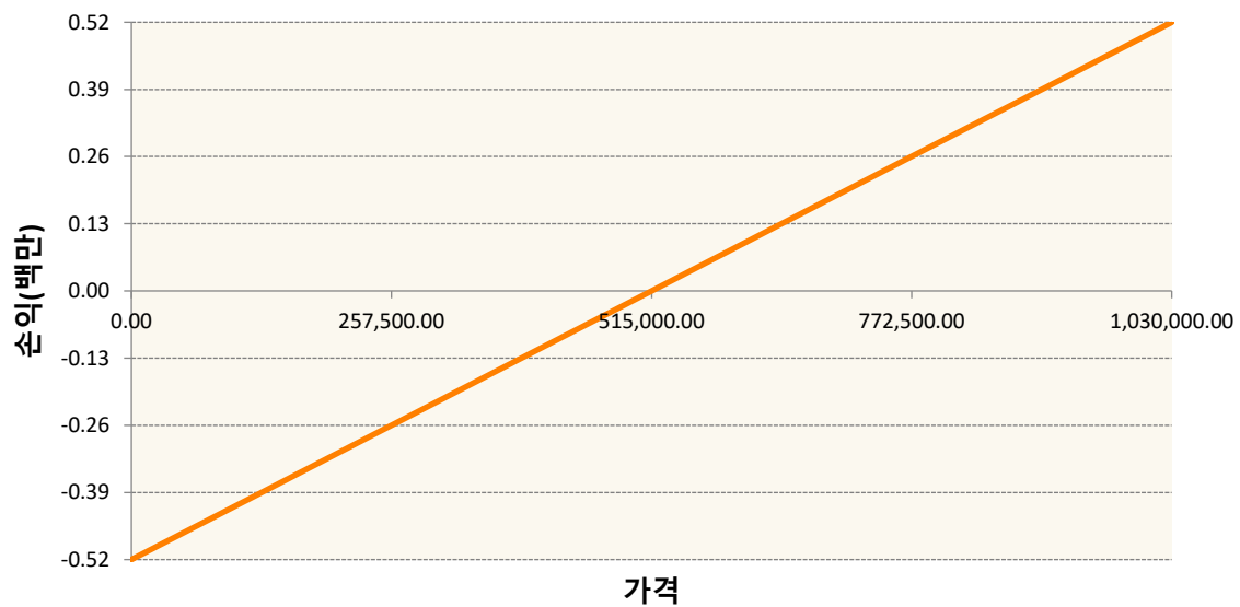
KR4147S70000-2022-07 LG화학개별선물
