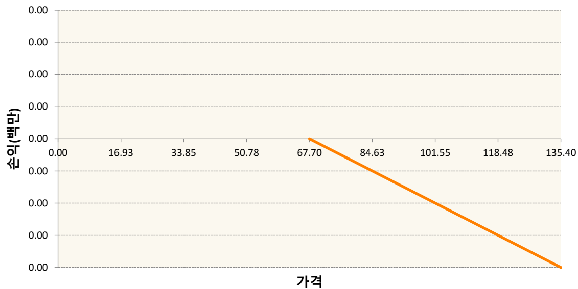
OESXN2-C3425-EURO STOXX 50
