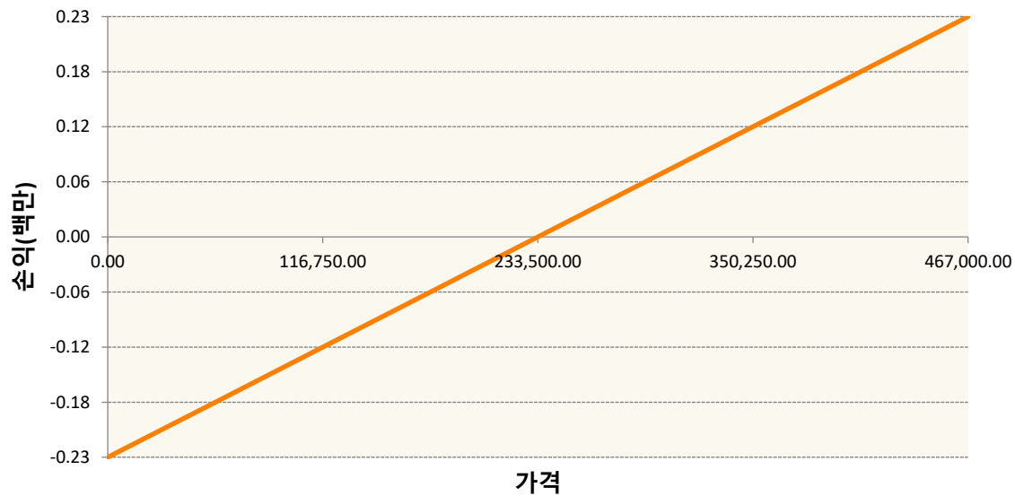
KR4156S80000-2022-08 NAVER개별선물
