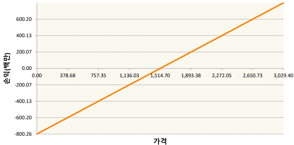
VNCH2-VN30 Index Future Mar22
