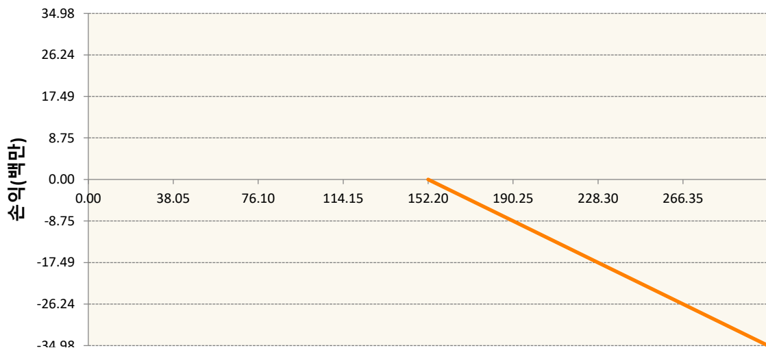
OESXF2-C4175-EURO STOXX 50
